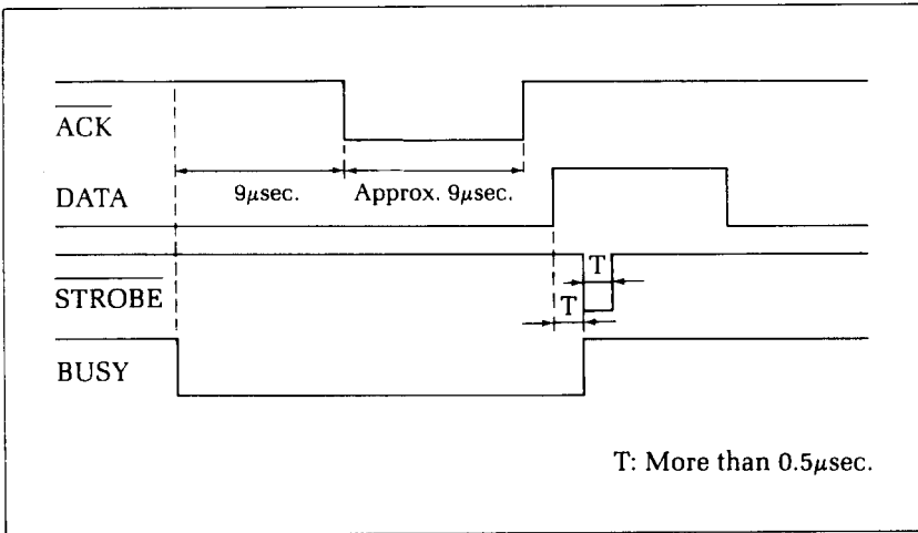
Figure H-1. SD-10/15 interface timing diagram.
