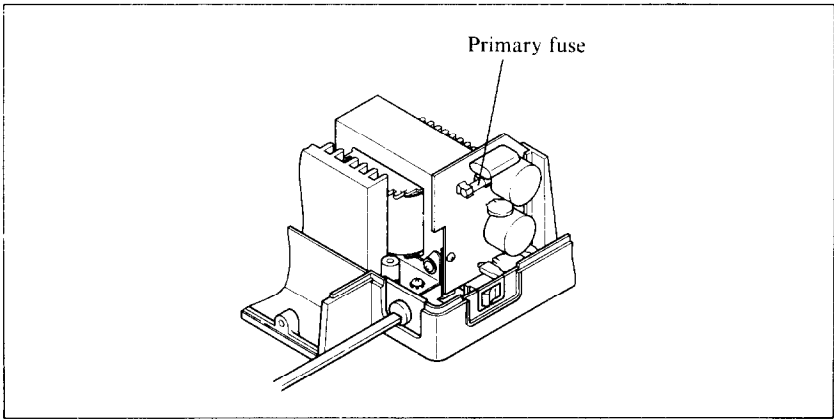
Figure 11-4. After removing the screws, pull the upper case slightly forward and lift it off the printer. The primary fuse is located near the power switch.
