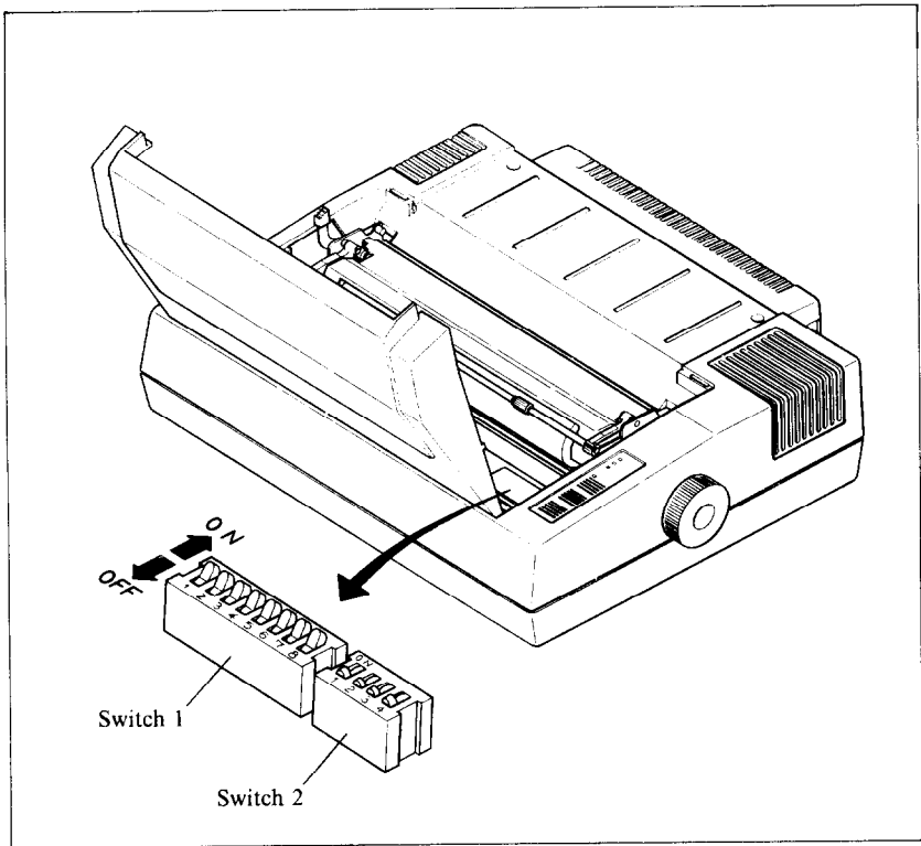
Figure A-2. SD-10/15's DIP switches are located under the printer cover.
