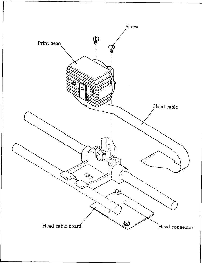
Figure 11-5. Replacement of SD-10/15's print head is simple.
